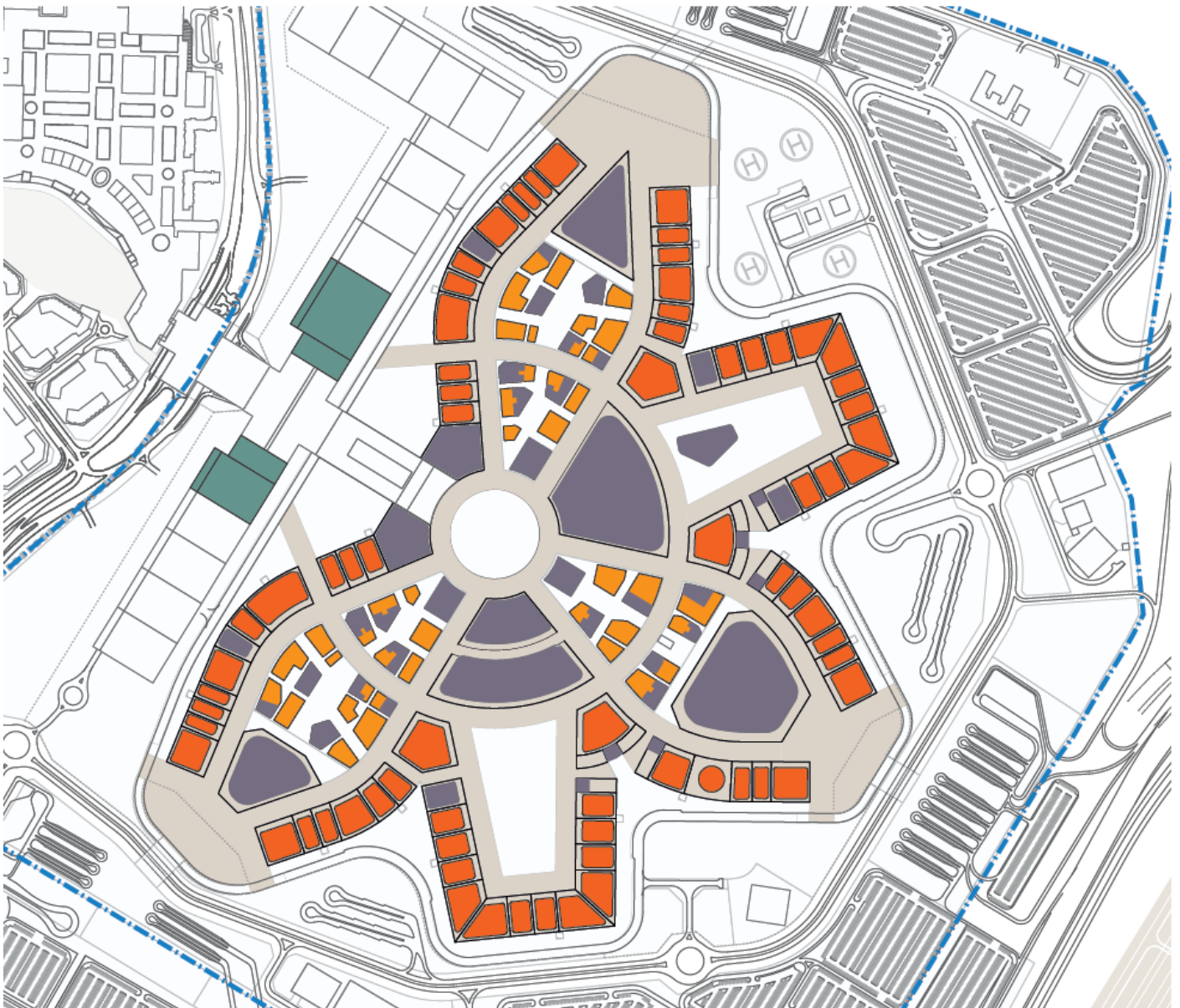
Figure 25 Building Typology Plan
